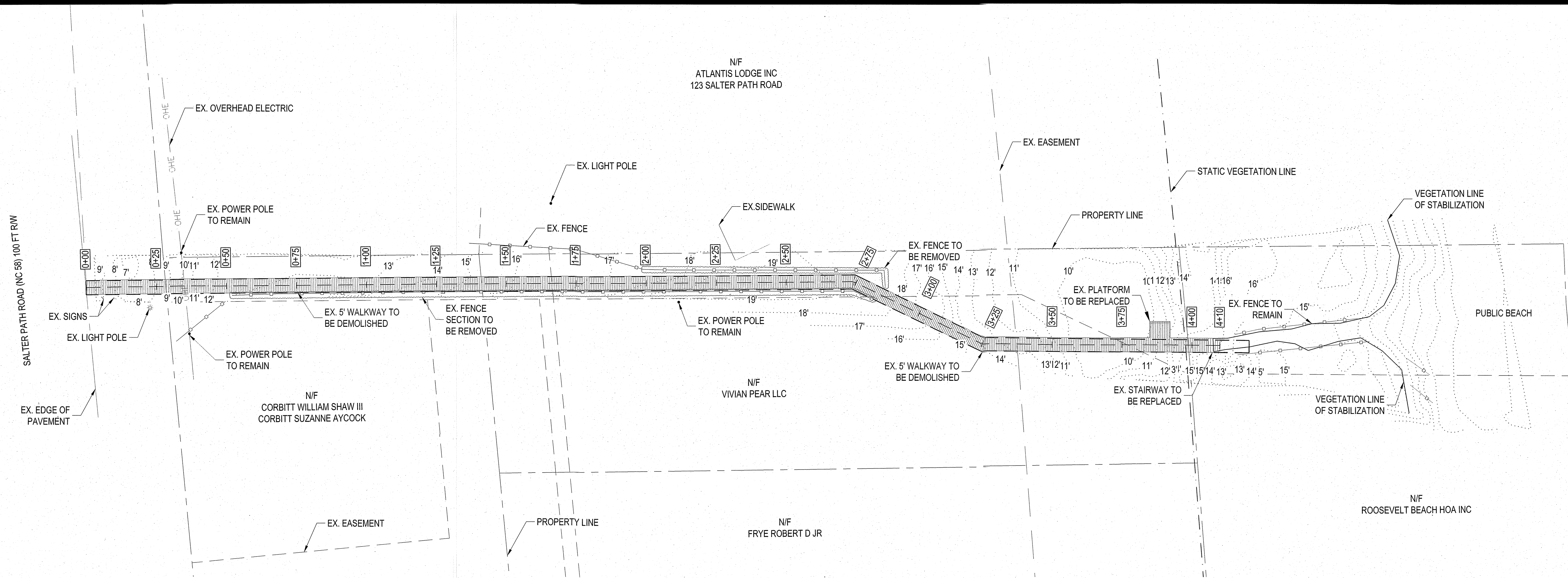
EXISTING CONDITIONS & DEMOLITION PLAN
