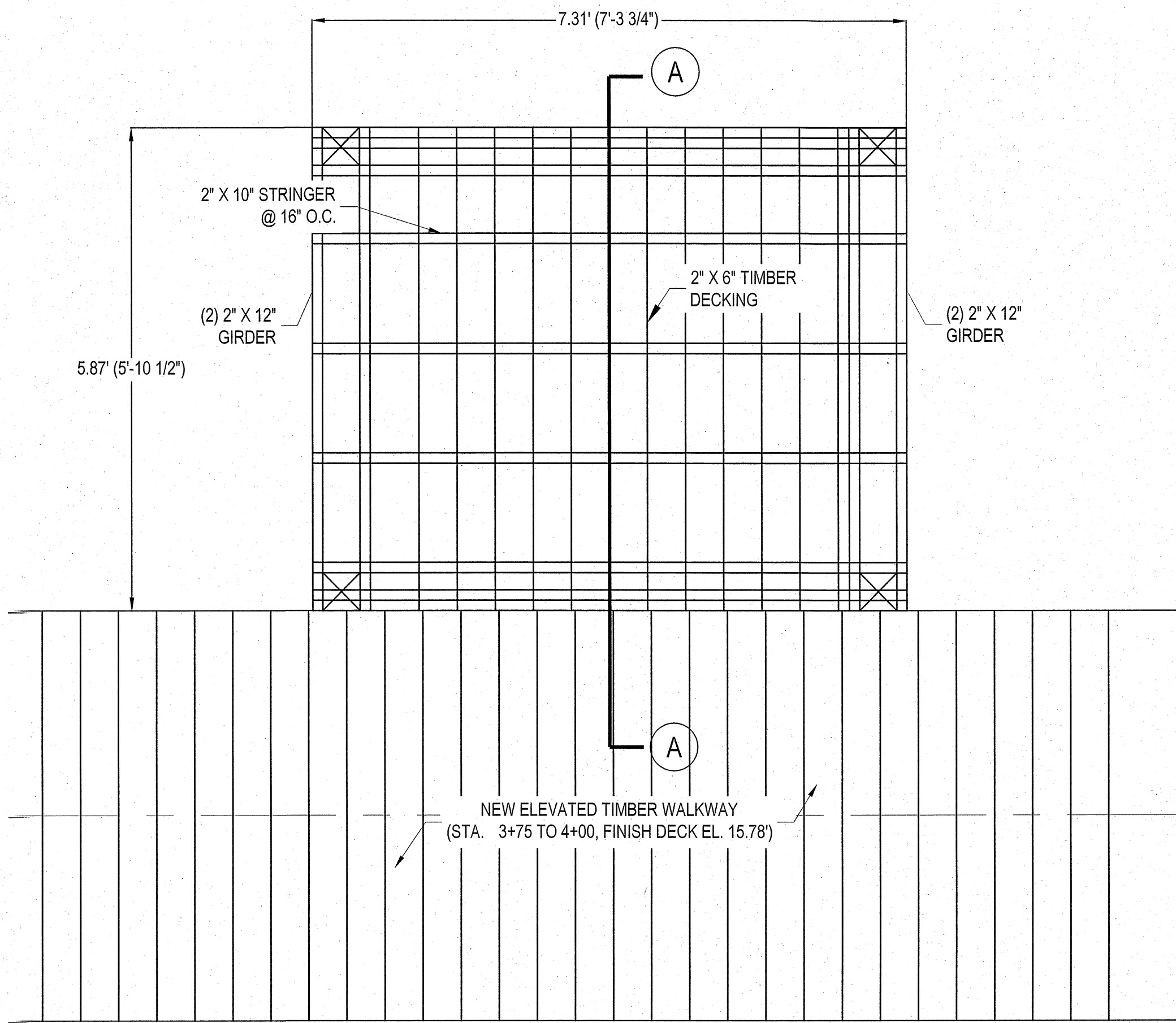
PLATFORM FRAMING & DECKING PLAN
