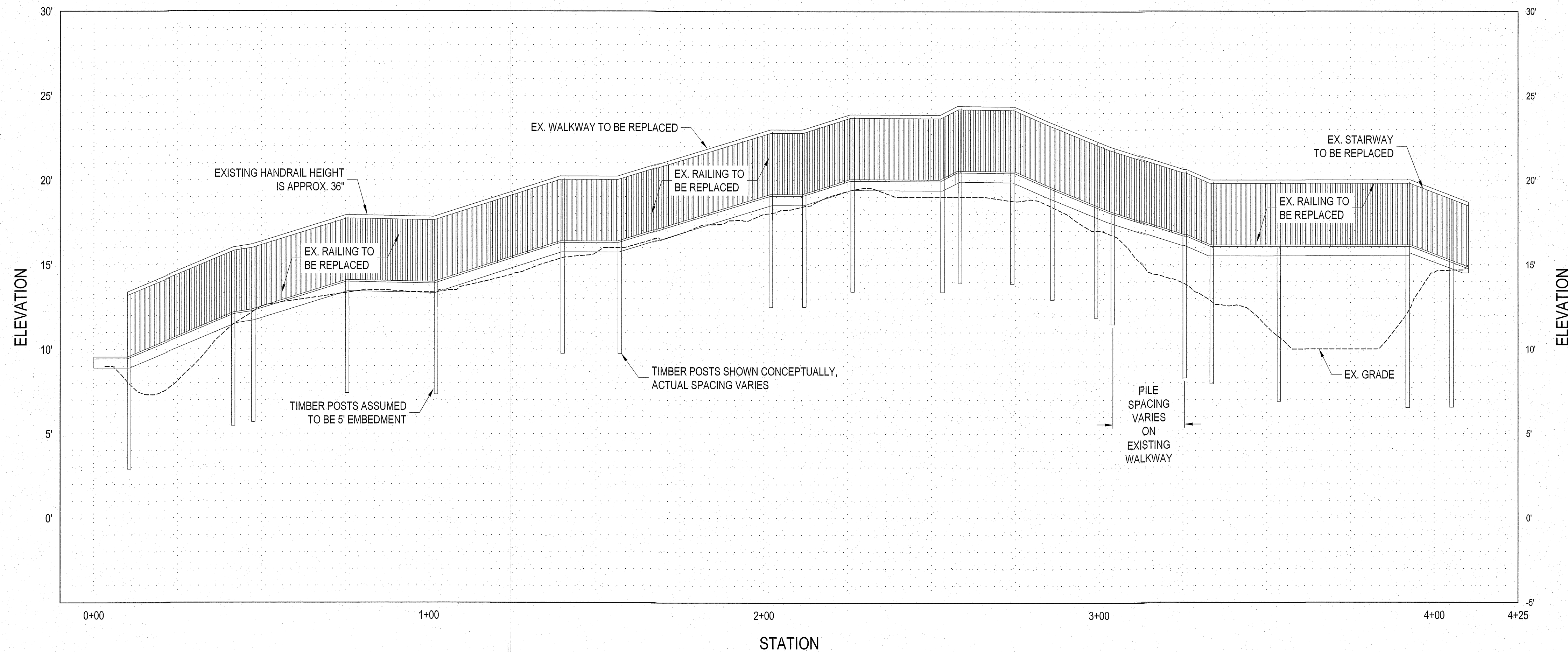
EXISTING CONDITIONS & DEMOLITION PROFILE
