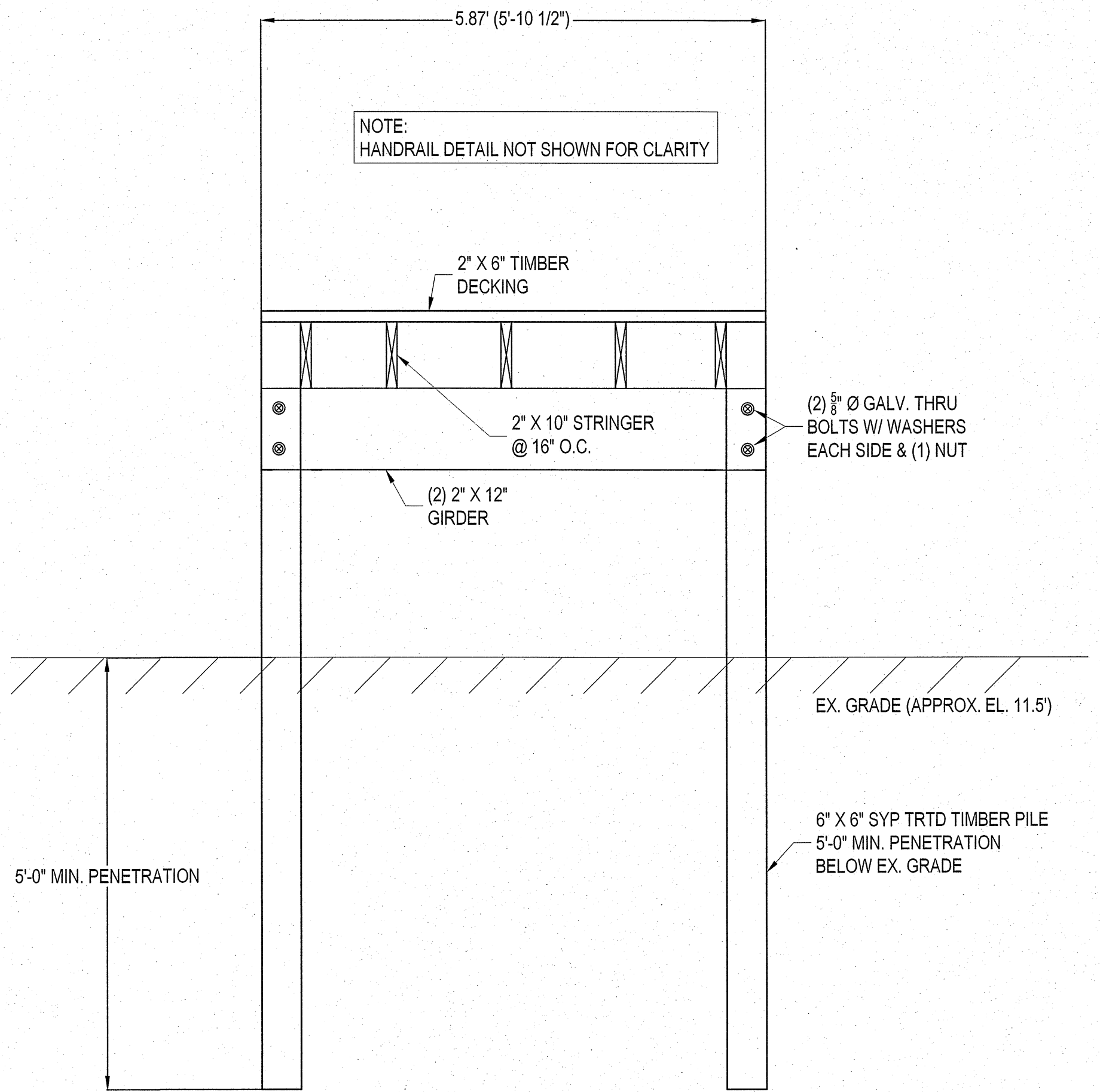
SECTION A-A: PLATFORM SECTION & ELEVATION
