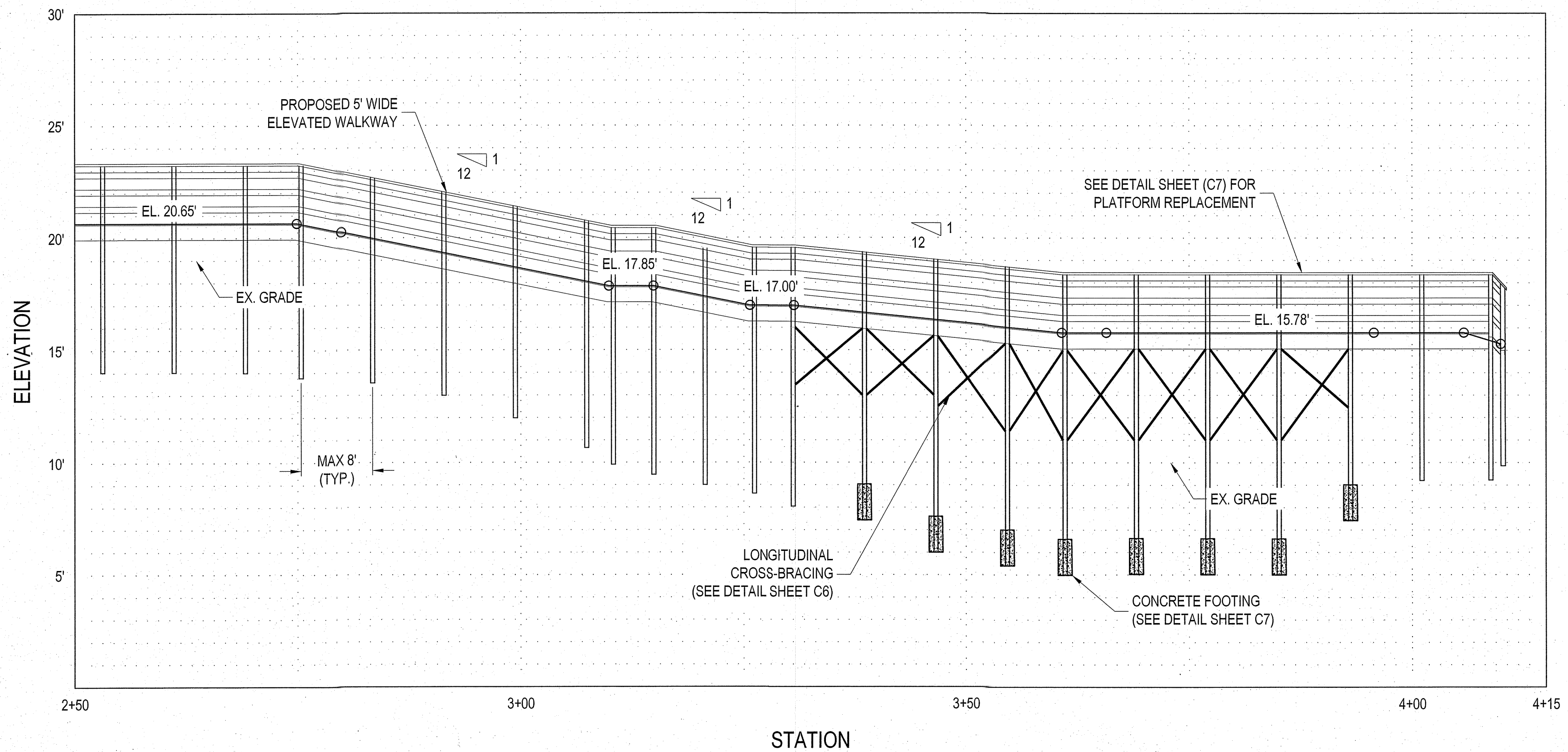
BOARDWALK PROFILE: STA. 2+50 TO 4+10
