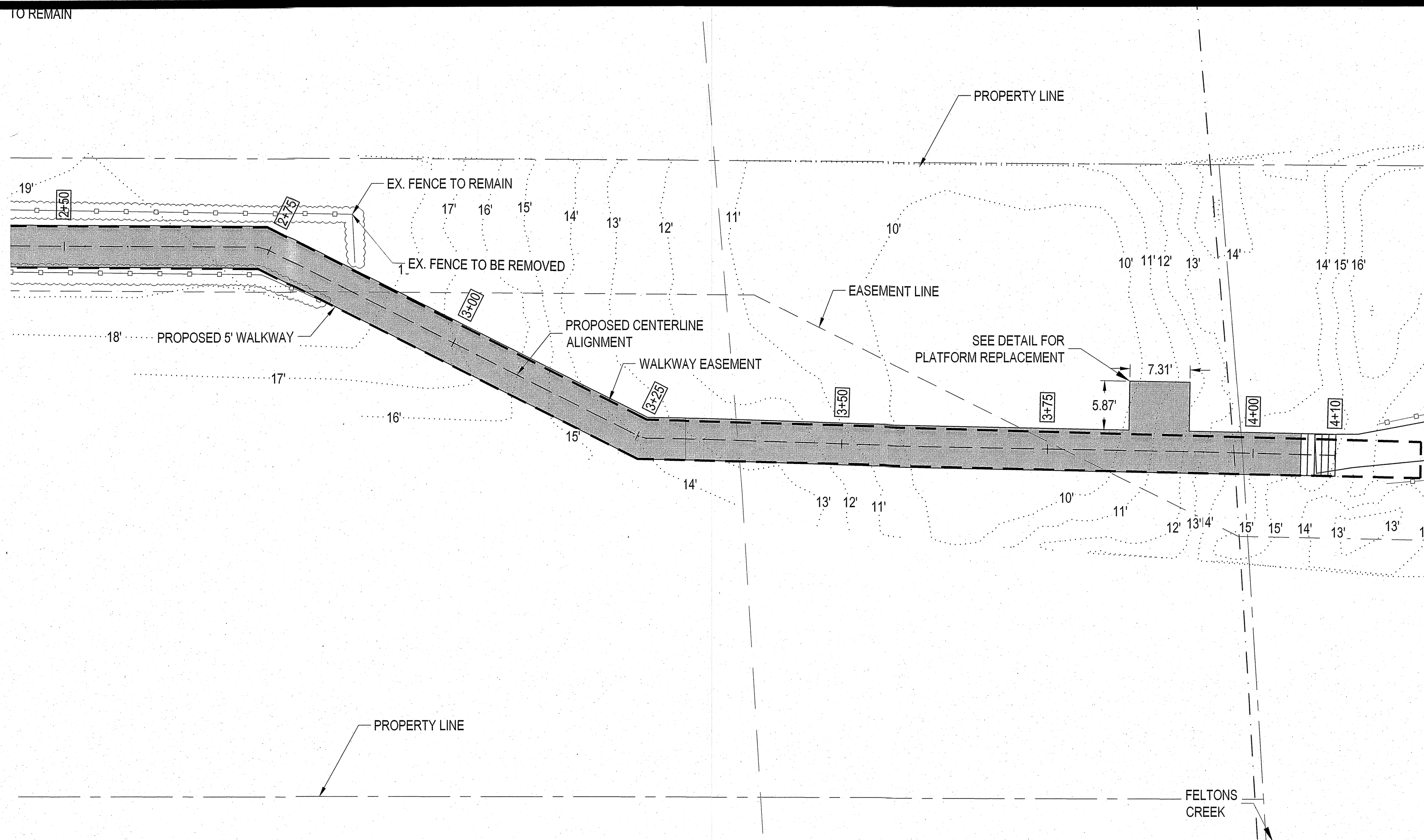
BOARDWALK PLAN: STA. 2+50 TO 4+10
