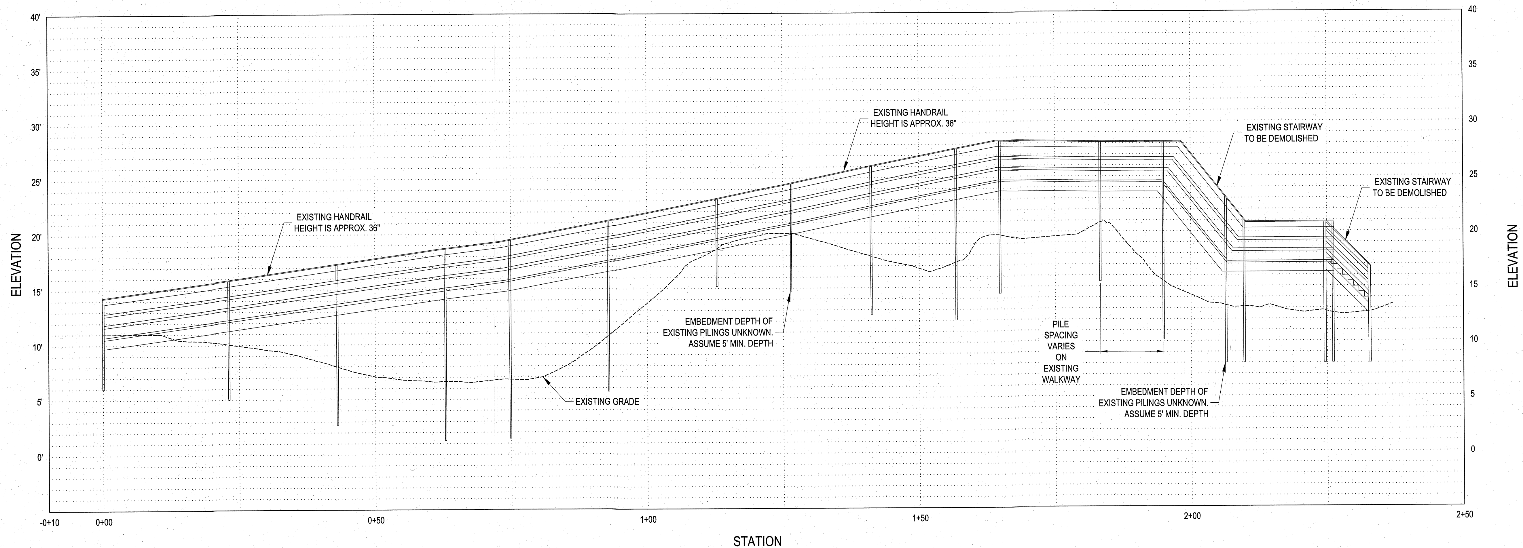
EXISTING CONDITIONS & DEMOLITION PLAN & PROFILE SCALE: 1" = 10'
