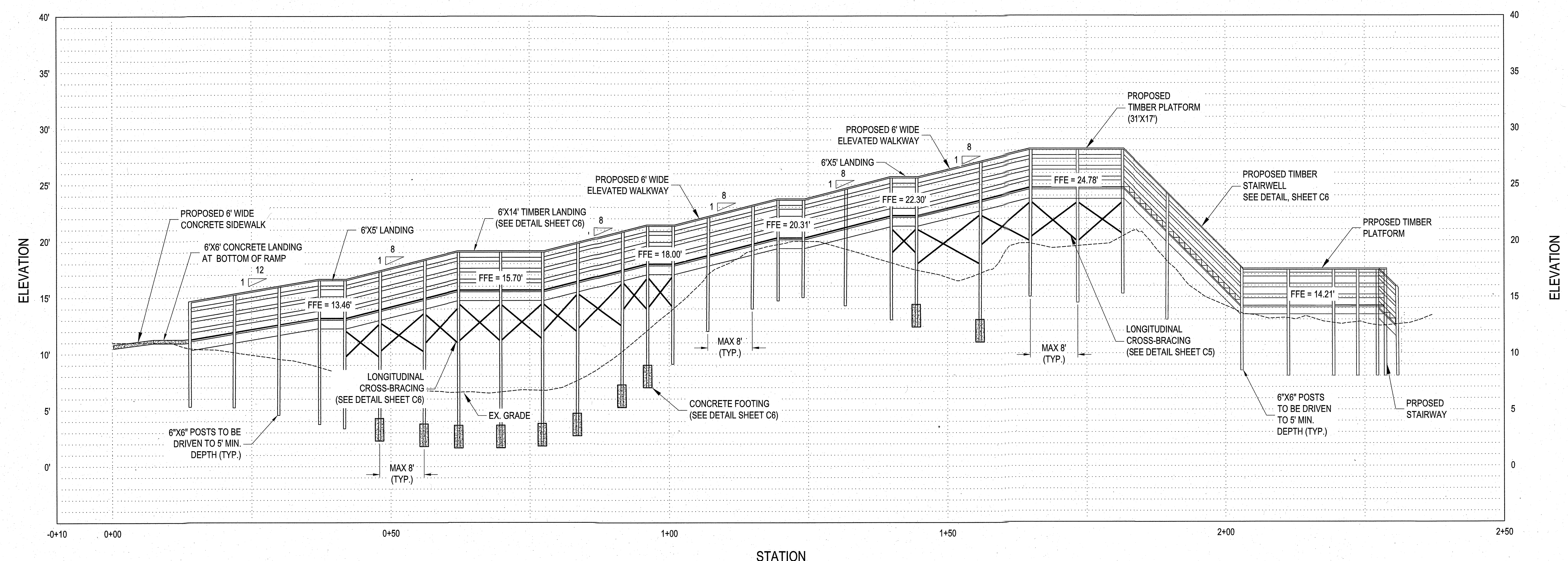
PROPOSED WALKWAY PLAN & PROFILE SCALE: 1" = 10'
